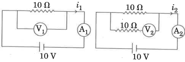
Circuit 1
